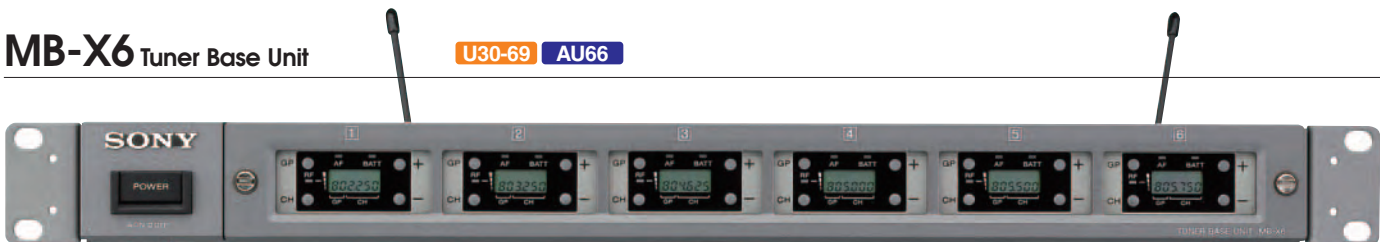
Front Panel: MB-X6 with six WRU-806A/806B tuner units installed
