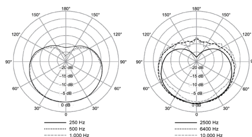
Typical Polar Pattern
