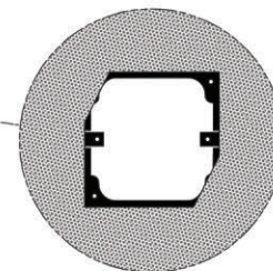
1-gang and 4 Sq mounting hole pattern
