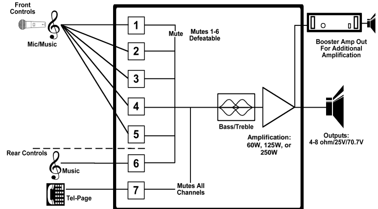
GTC Series Mixer Amplifier
