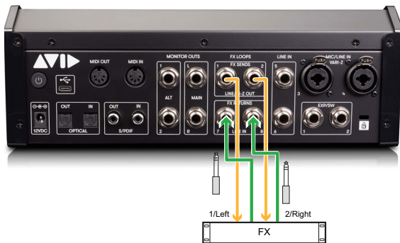
Connecting a stereo rack mount effects processor
