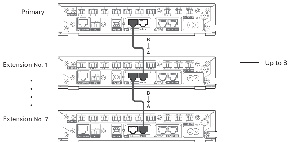
Connection example
