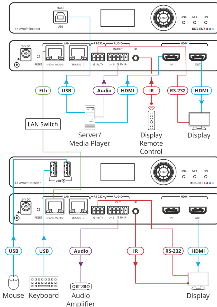
Figure 3: Connecting the KDS-EN7 and KDS-DEC7
