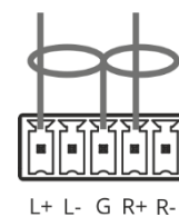
Figure 5: Connecting to an Unbalanced Stereo Audio Acceptor
