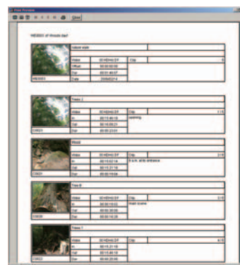
Print Function
