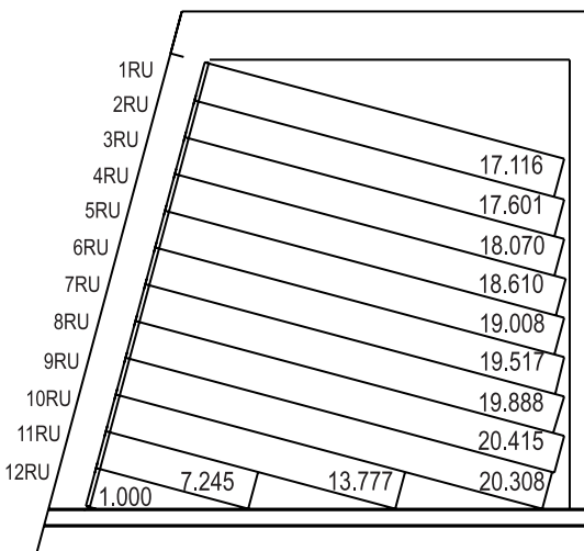
Maximum racking depth for each rack unit on 15° slope
