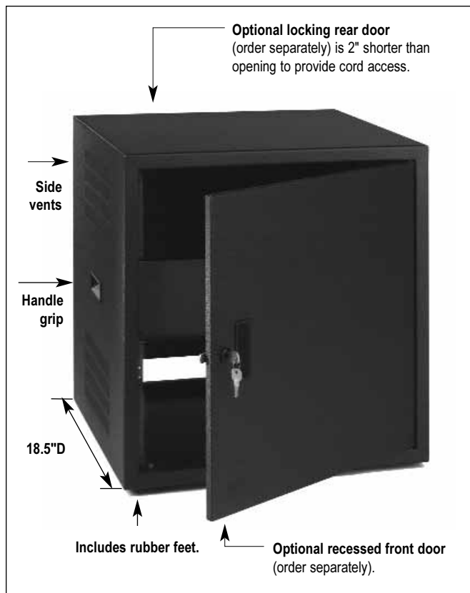
L70 Series desktop cabinets Model L70-24 shown with optional front door Model L151-24 and optional rear door Model L7-1922
