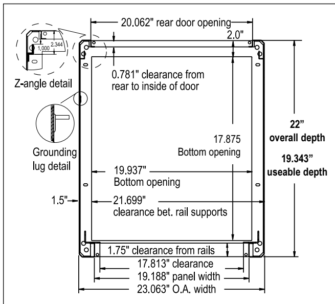
BOTTOM FOOTPRINT & CABINET CROSS-SECTION (see tech sheet #1AT-100 for seismic base detail)
