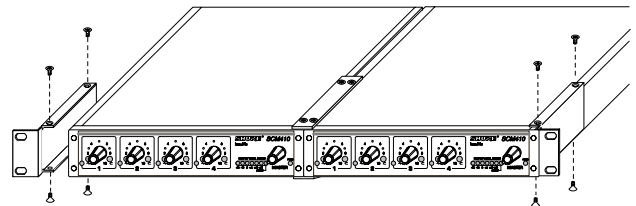
INSTALLING FULL-RACK MOUNTING BRACKETS
