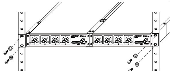
RACK MOUNTING DUAL SCM410/E MIXERS
