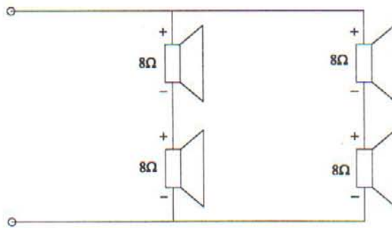
Figure 4c: Series Parallel Combination: 8Ω
