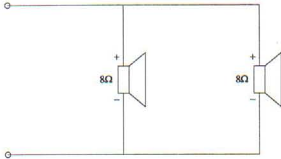
Figure 4a: Simple parallel connection: 4Ω
