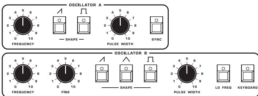
The Oscillators section
