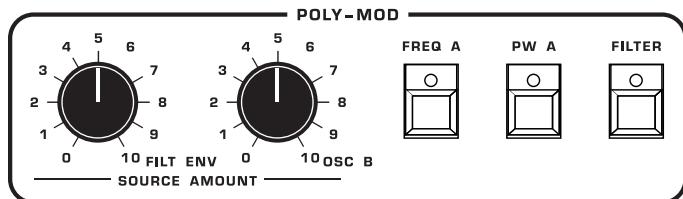
The Poly Mod section
