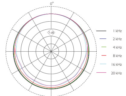
Typical directional characteristics of a 4661 Heavy Duty
