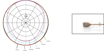
Polar Pattern of d:fine™ Omnidirectional
