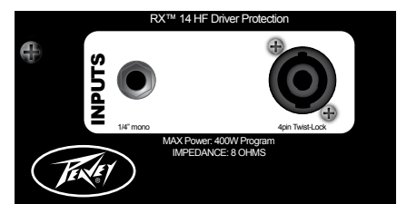
PVX 12 Input Plate
