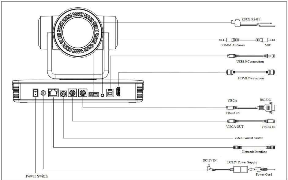
Figure 2.5 Wiring Diagram
