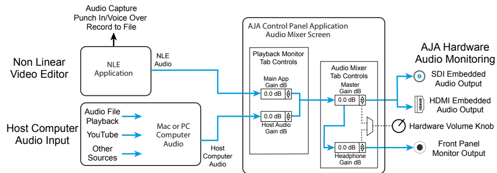
Figure 8. T-TAP Pro Audio Monitoring Routing Diagram
