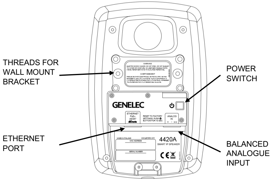
Figure 3. Connectors and controls in the 4420A rear panel.
