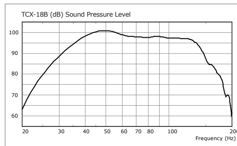
Frequency Response
