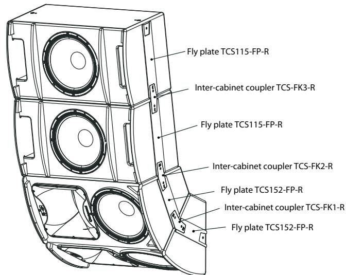
Vertical array using fly plates and inter-cabinet couplers on left and right.
