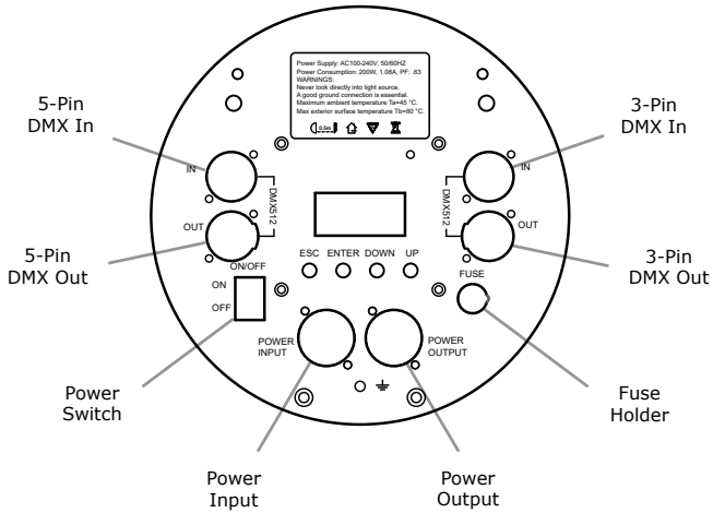
Figure 2: The Rear Connections
