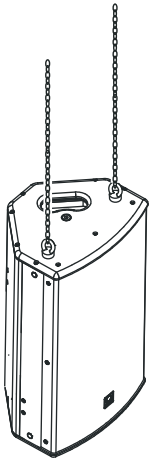
Suspension using M10 shoulder eyebolts
