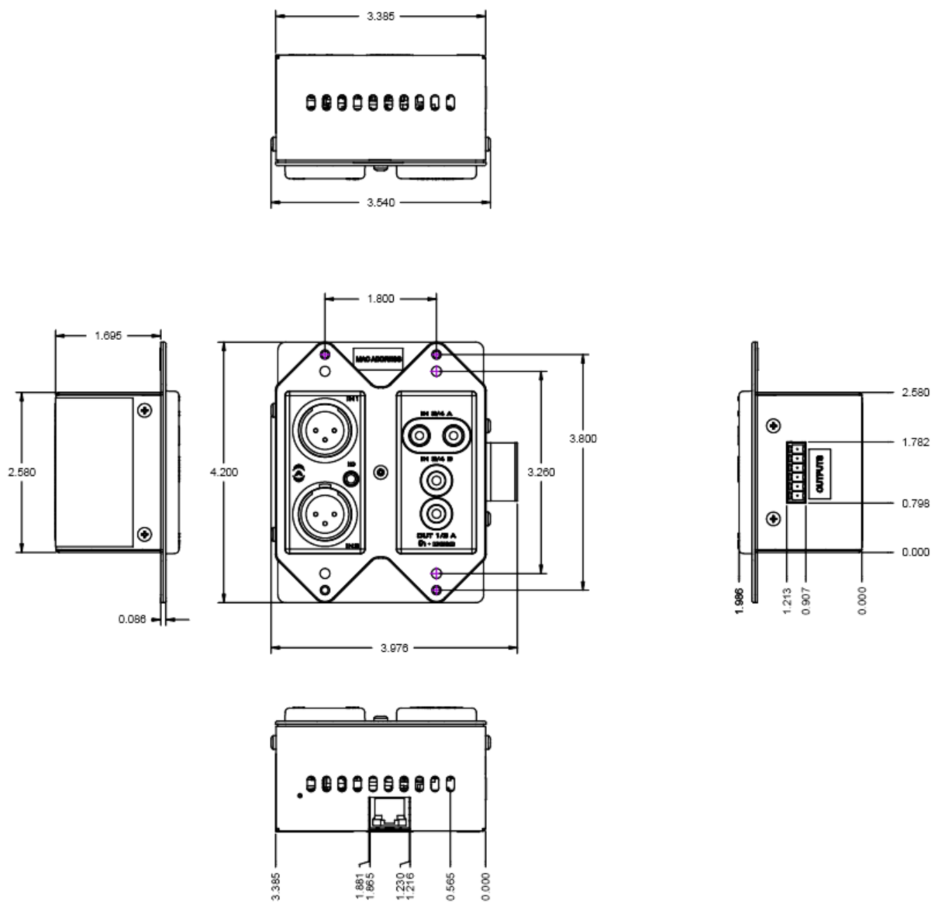
Figure 4 - Dimensioned Drawing
