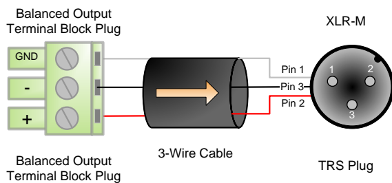
Figure 5 - Balanced Wiring Guide
