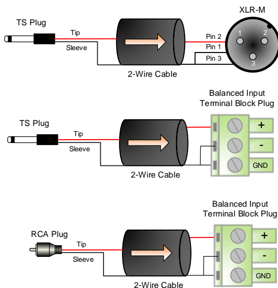
Figure 6 – Unbalanced Wiring Guide
