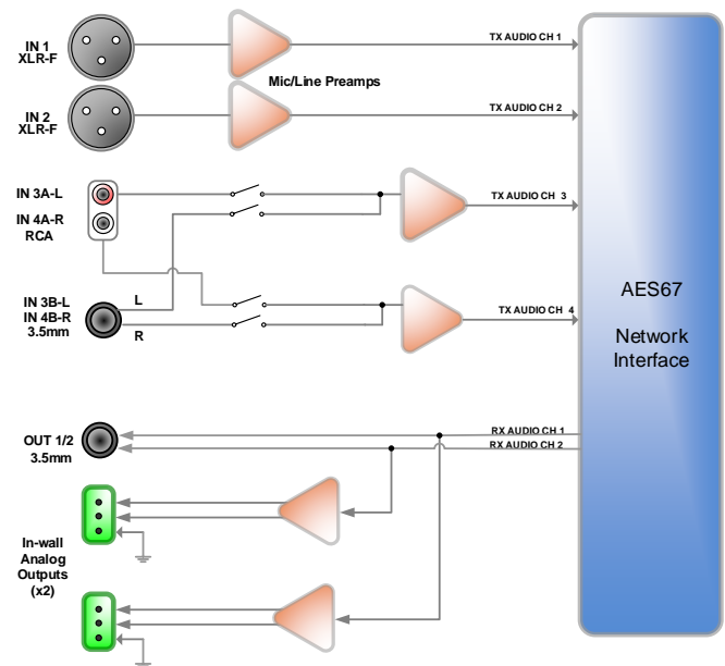
Figure 2 - unA610 Signal Flow
