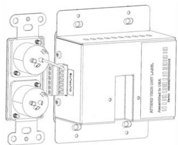
Figure 3 - unA6IO Installed with unXP2O (Rear View)
