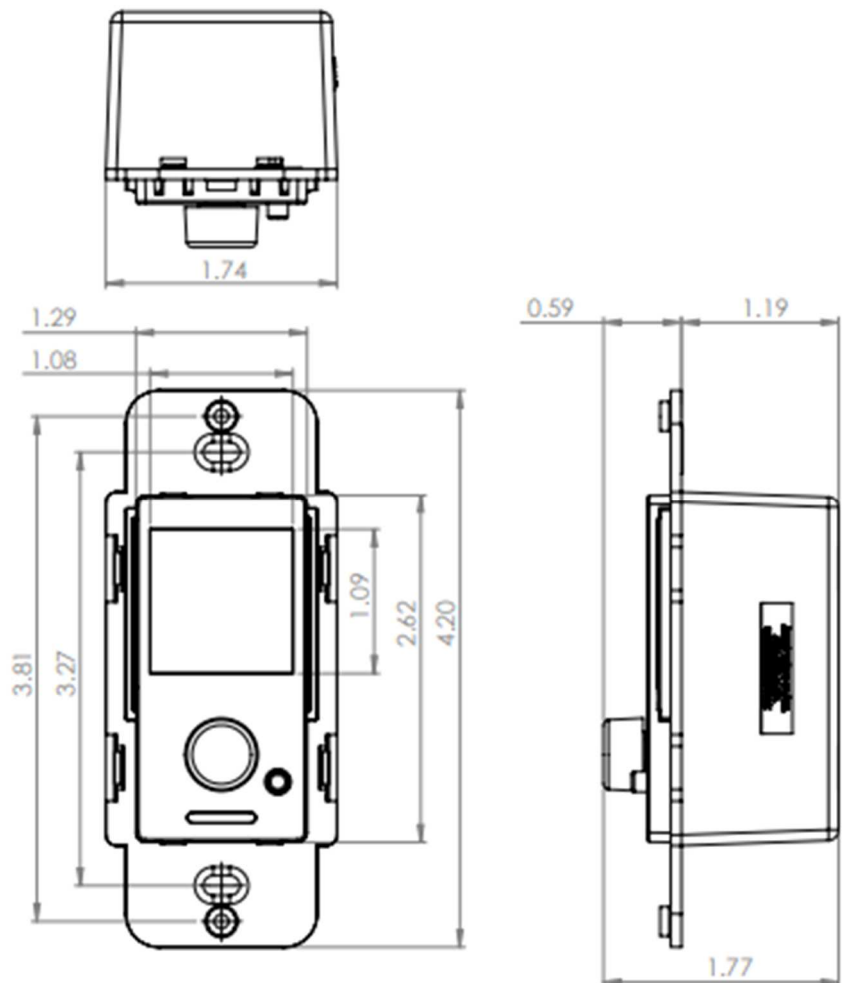
Figure 3 - Dimensional Drawing
