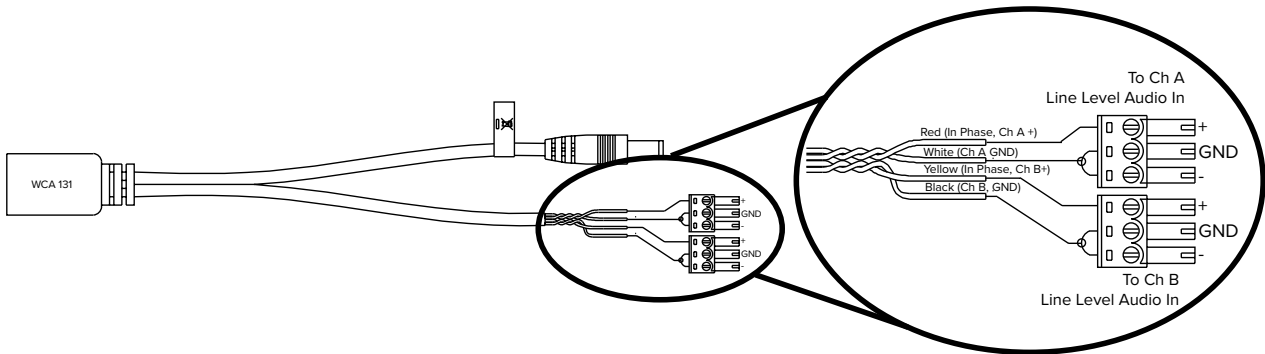
Figure 9: Unbalanced Line Level Audio Output
