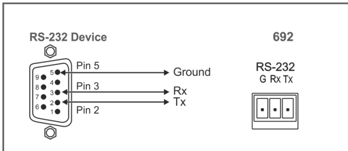
Figure 7: RS-232 Connection
