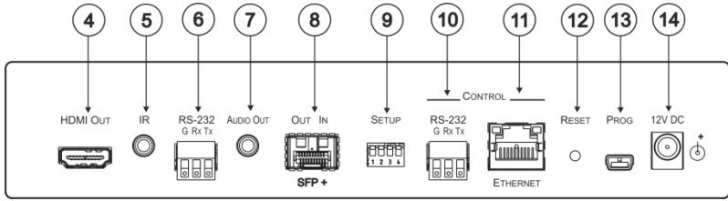
Figure 2: 692 Rear Panel
