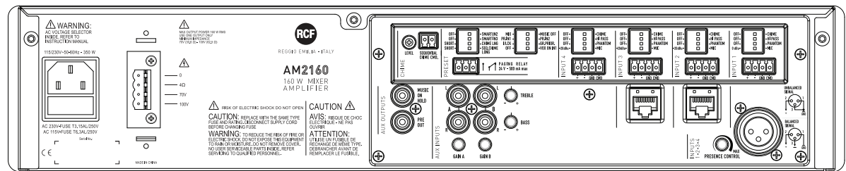
Rear panel
