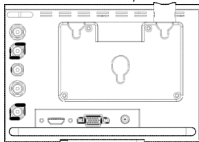
TLM-700HD-A with Anton Bauer Battery Mount
