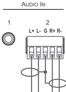
Figure 7: Connecting a Balanced Stereo Audio Source to the Balanced Input
