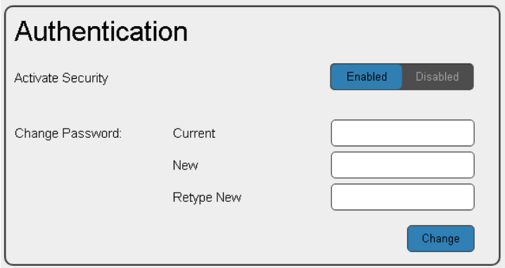
Figure 23: Authentication Page
