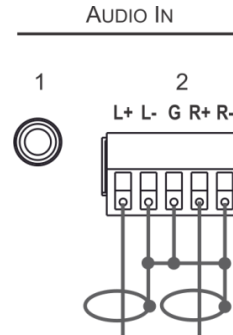
Figure 8: Connecting an Unbalanced Stereo Audio Source to the Balanced Input
