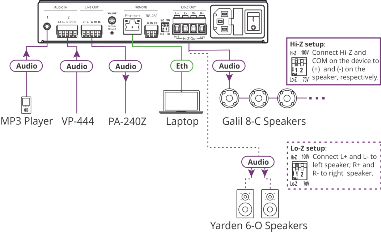
Figure 4: Connecting to the PA-240Z Rear Panel
