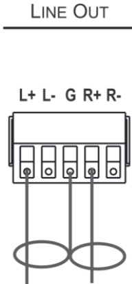
Figure 6: Connecting to an Unbalanced Stereo Audio Acceptor
