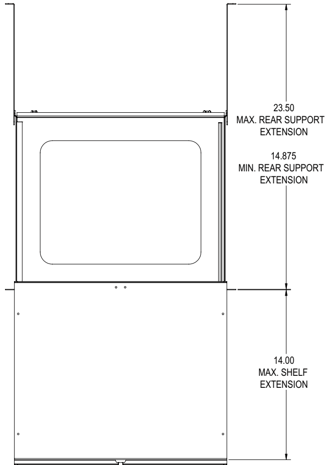
TOP VIEW FULLY EXTENDED
