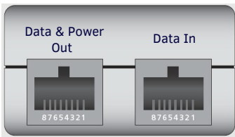
FIG. 8 POE INJECTOR CONNECTION
