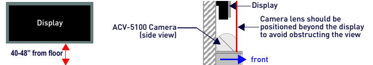
FIG. 4 ACV-5100 WALL MOUNT CONSIDERATIONS
