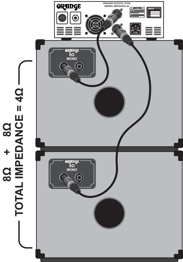
ORANGE BASS AMPS = MIN 4\Omega
