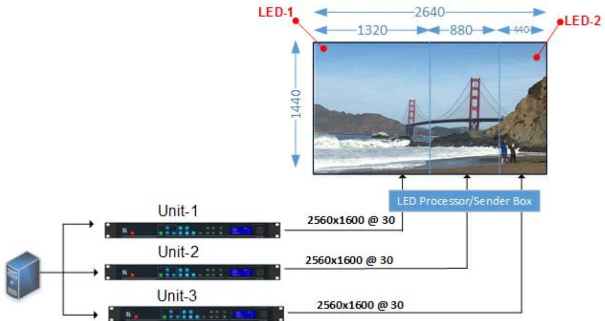
Figure 8: Advanced Splicing - 3x1 example
