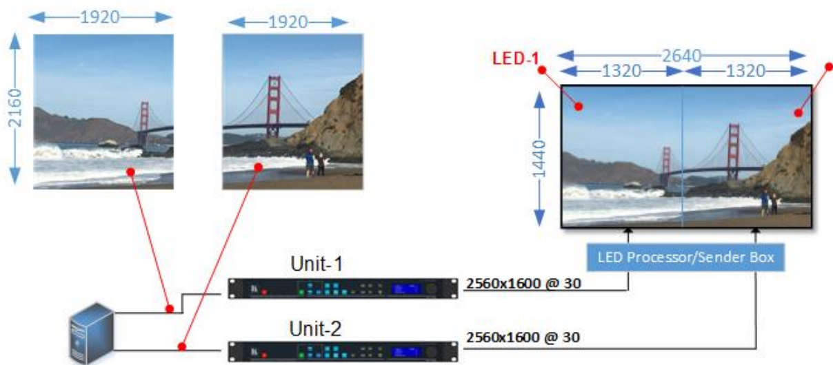
Figure 5: Standard Splicing - 2x1 example (pre-split source)
