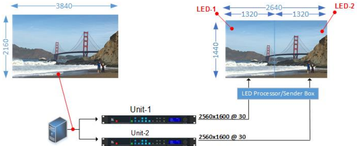
Figure 6: Standard Splicing - 2x1 example (common source)
