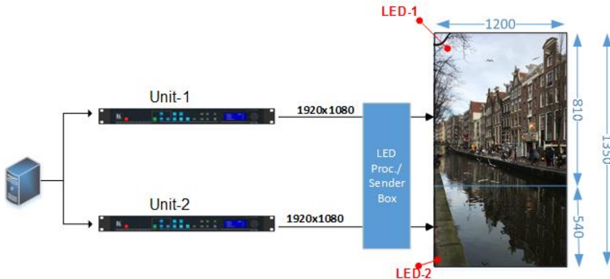
Figure 9: Advanced Splicing - 1x2 example
