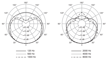
FP2/SM58 Polar Pattern
