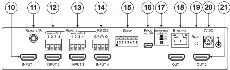
Figure 2: VS-42UHD 4x2 HDMI Matrix Switcher Rear
