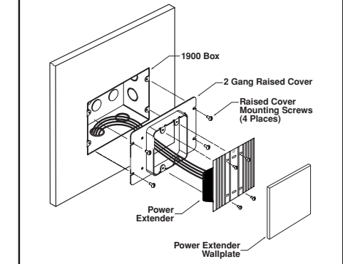
Figure 1B: Flush Mounting
