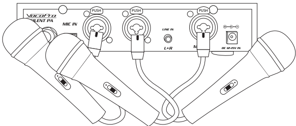
Illustrations shown with XLR connections. Microphones with 1/4" cables can also be connected to the MIC IN and LEFT/RIGHT XLR-1/4" Combo Jacks.
