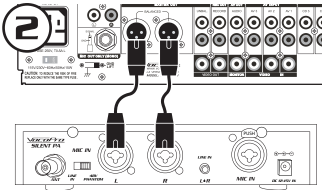
Illustration shown using XLR cables. Connection can also be made using 1/4" Stereo Cables
