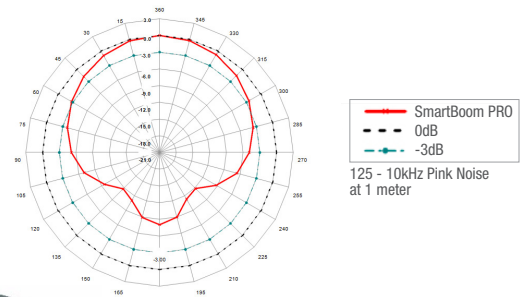
Microphone Polar Pattern
