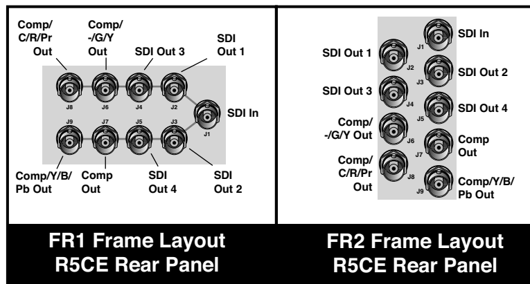
FR1 and FR2 BNC Connector Assignments, R5CE Card Module
