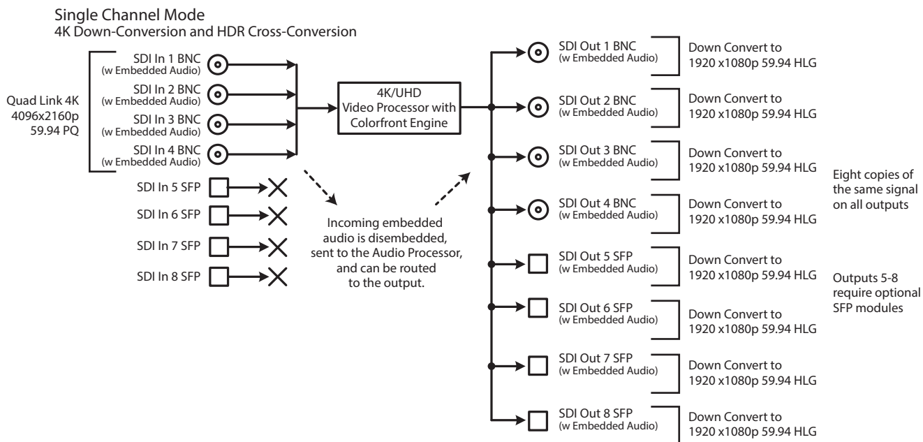
Figure 5. Single Channel Mode, Down and HDR Cross-Conversion
