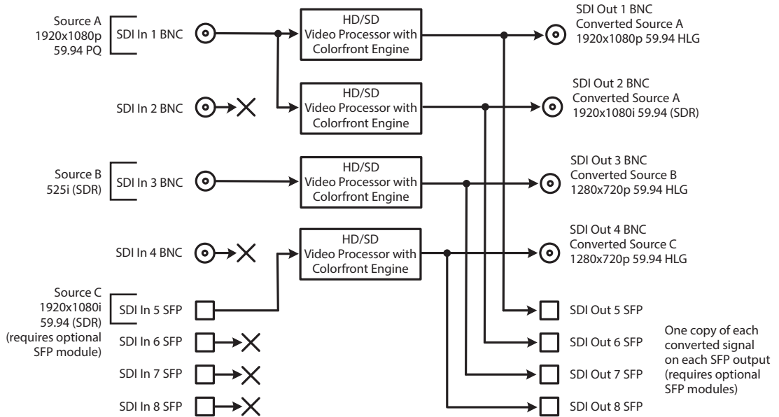
Figure 7. Four Channel Mode Example, Four Conversions of Three Sources
