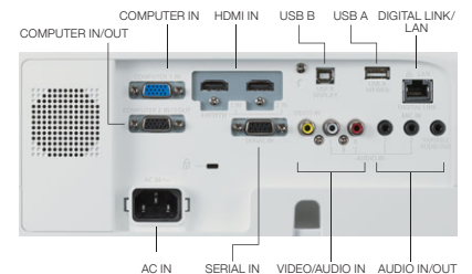
Terminal layout for PT-VZ575N/VW535N/VX605N.
