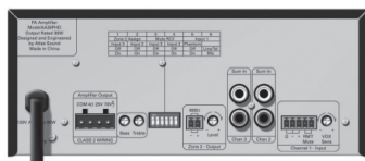
AA30PHD - REAR
