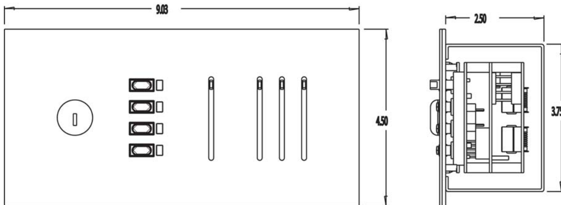
3 Preset/3 Fader w/Master/Lockout & Off Shown in Drawing Above
