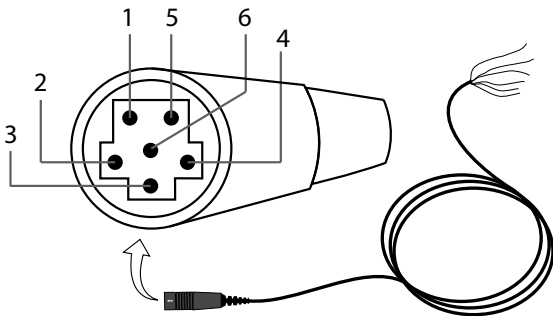
6-Pin Headset Connector
