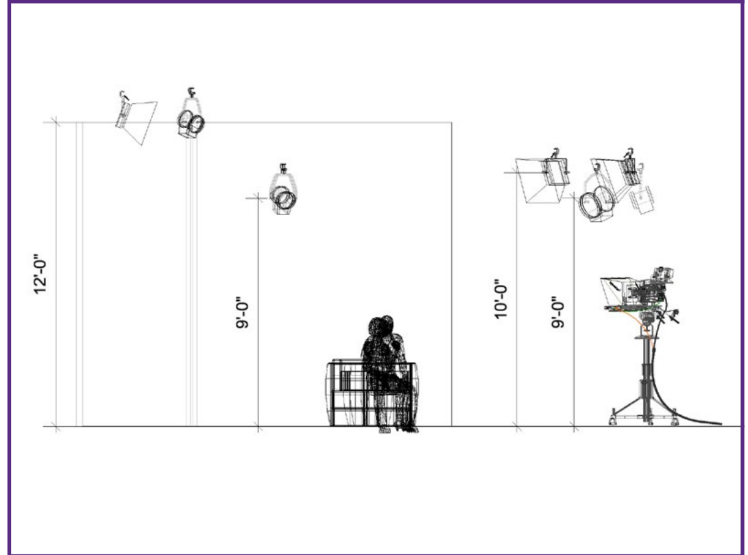
SECTION VIEW
