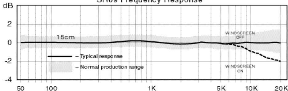
SR69 Frequency Response
