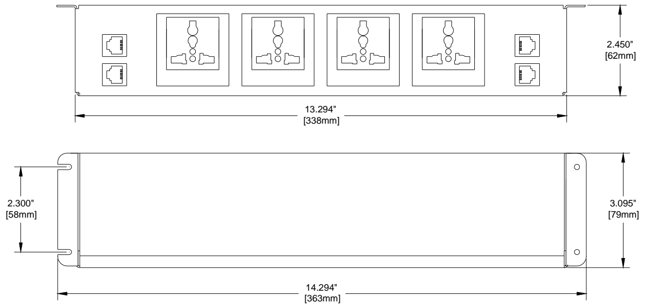
Diagram 13: UT240-551 Universal
