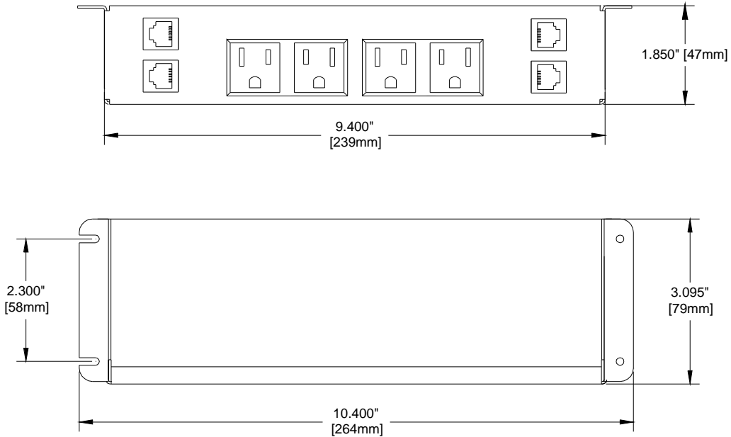
Diagram 5: UT240-313 U.S./Canada
