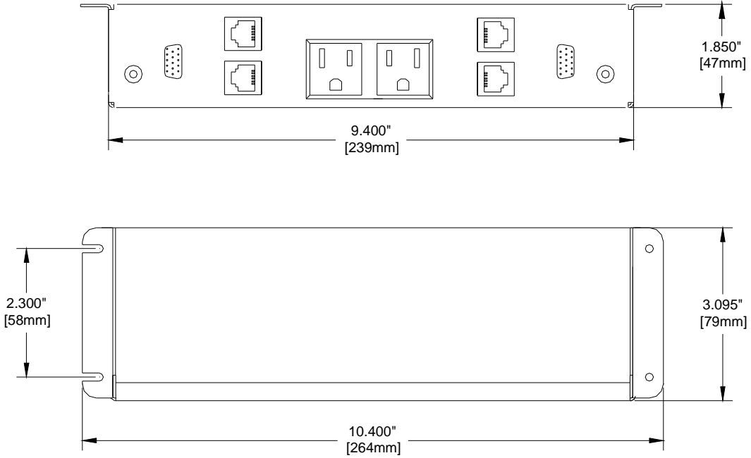
Diagram 3: UT240-311 U.S./Canada
